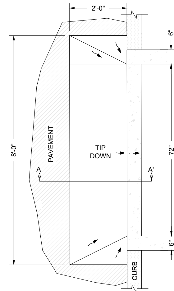
PLAN VIEW
