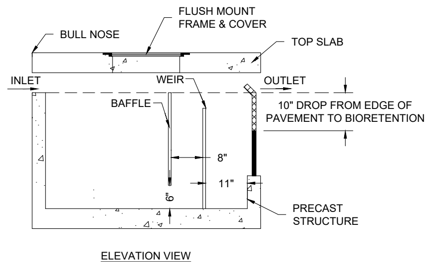
PRETX 48X48 UNIT DETAIL
