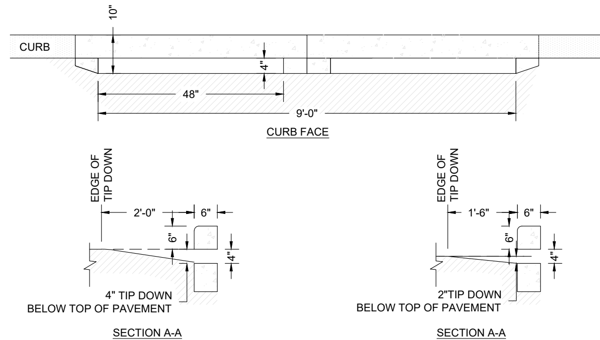
PRETX 6" CURB REVEAL DETAIL
